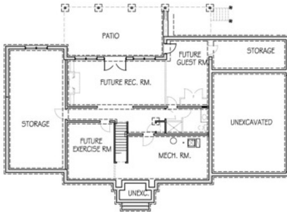
BASEMENT PLAN
